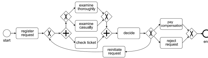
Fig. 3: Example process model in BPMN notation, adopted from (van der Aalst, 2016). The model describes process behavior in terms of the same high-level business activities as presented in the event log in Table 1.
