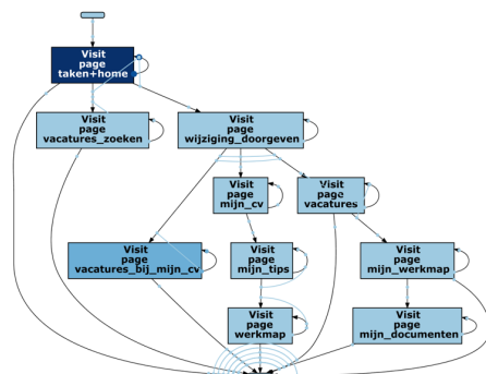
(b) Automatically discovered process model using the clickstream data abstracted into coarser granularity. The model provides much more insights into the high-level user-behavior.
